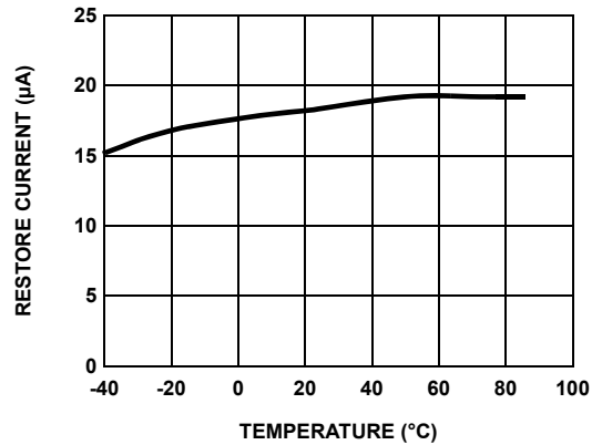
FIGURE 18. DC-RESTORE CURRENT vs TEMPERATURE
