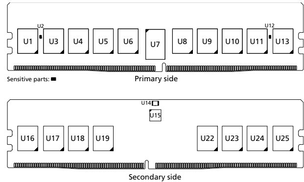
Figure 1: 288-Pin DDR5 RDIMM (R/C-F0)
