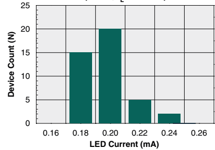
Typical I_F for Switch Dropout (N=50, I_L=400mA )
