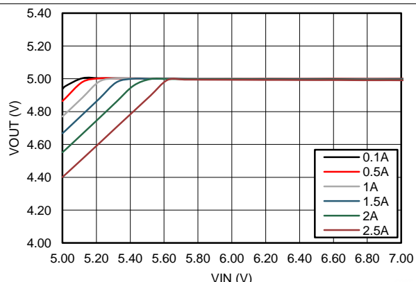
Figure 14. Dropout Curve V_{OUT} = 5\text{ V} F_S = 200\text{ kHz}
