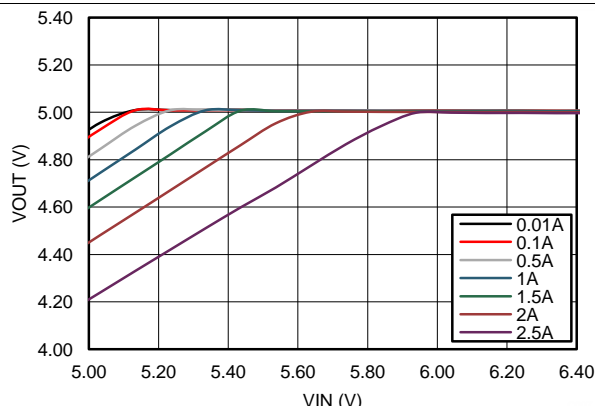
Figure 15. Dropout Curve V_{OUT} = 5\text{ V} F_S = 500\text{ kHz}
