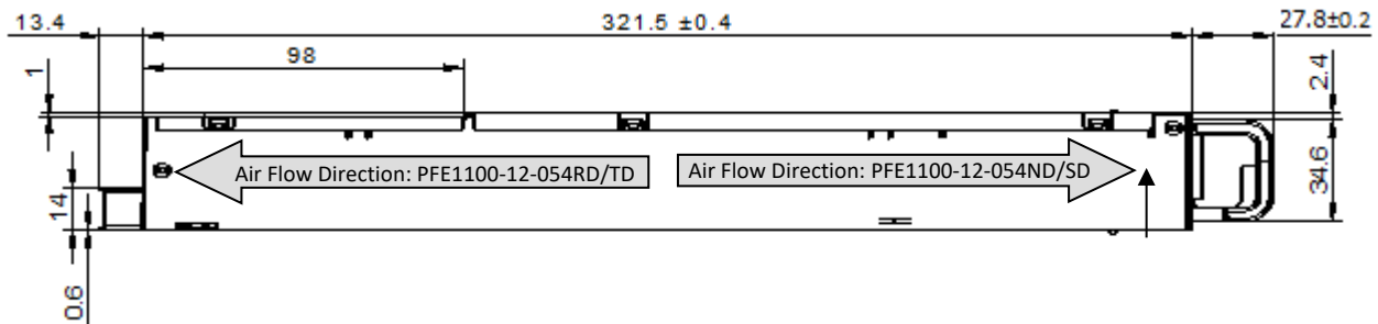
Figure 3. Side View 1
