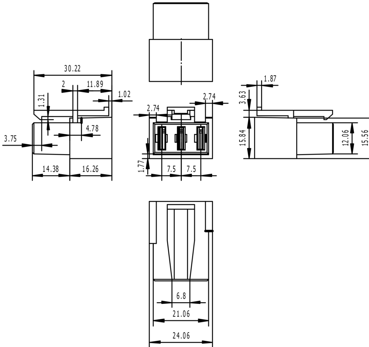
Picture 8. Receptacle: DP5ZJW0300-001
