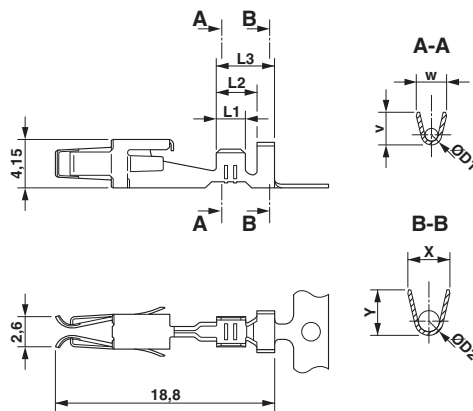
Dimensioned drawing
