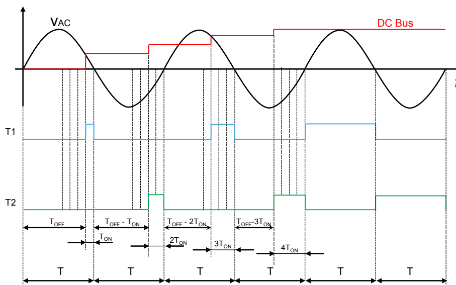
Figure 17. Digital Inrush Current Limiter function: sequence of driving of the SCR
