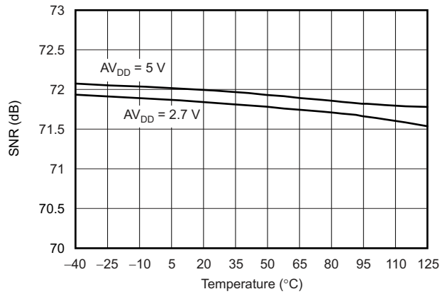
Figure 21. SIGNAL-TO-NOISE RATIO vs TEMPERATURE
