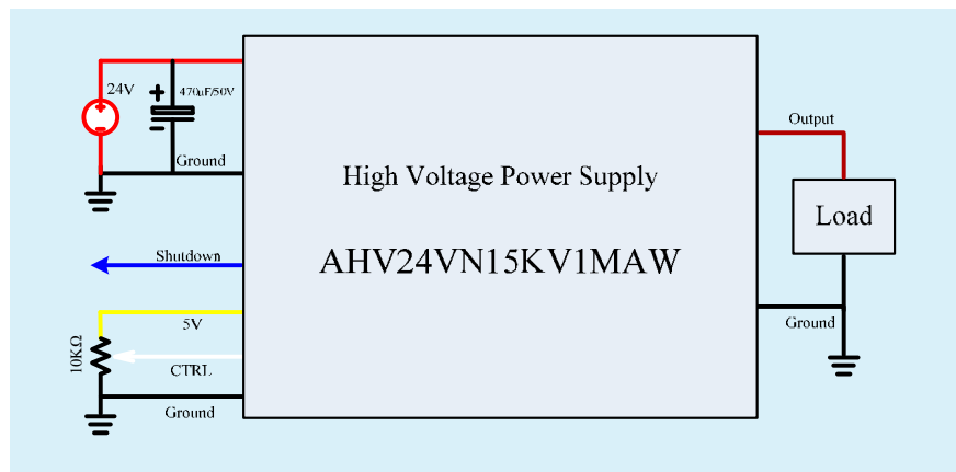
Figure 8. Control by External Signal Source
