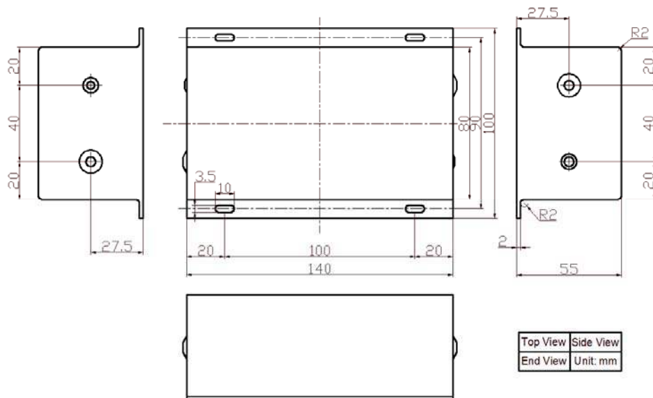
Figure 11. Dimensions for AHV24VN15KV1MAW
