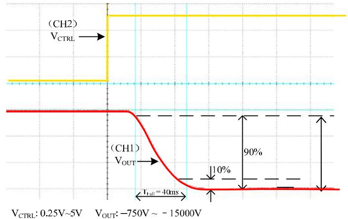
Figure 7. Fall Time
