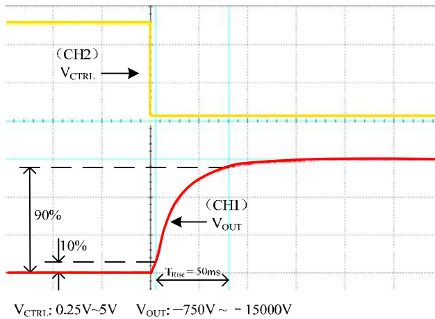
Figure 6. Rise Time
