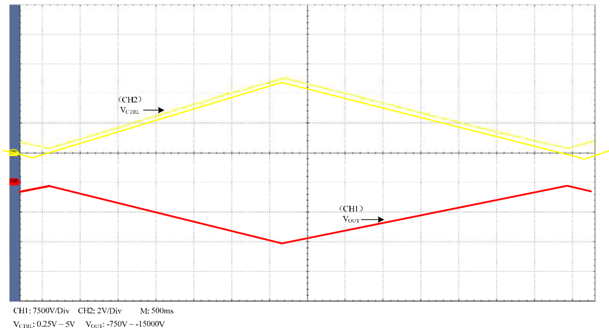
Figure 3. Triangle Wave
