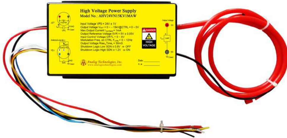
Figure 10. Leads of AHV24VN15KV1MAW
