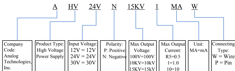
Figure 9. Naming Rules of AHV24VN15KV1MAW
