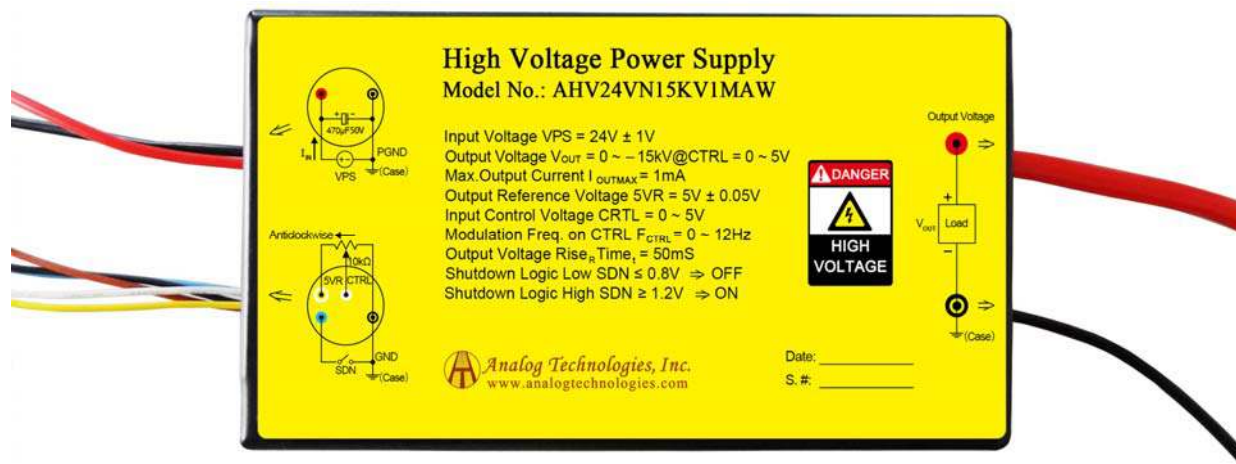
Figure 1. Physical Photo of AHV24VN15KV1MAW
