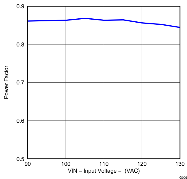
Figure 5. TPS92070EVM-682 Power Factor with Respect to Line Voltage, No Dimmer
