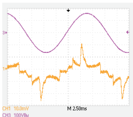
Figure 9. Input AC Voltage and Current, Full Load, No Dimmer (CH1 = I_{IN} , CH3 = V_{IN} (115 VAC), scale = 100 mA/div)
