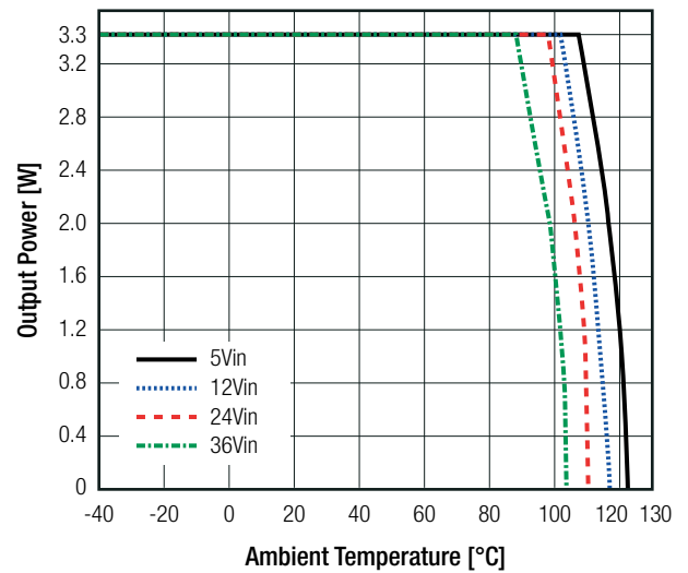
Thermal Derating
