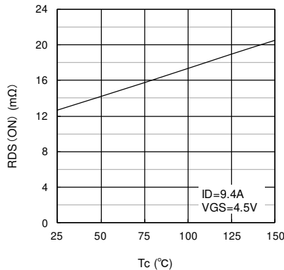
RDS(ON)-Tc characteristics (typical) ID=9.4A, VGS=4.5V
