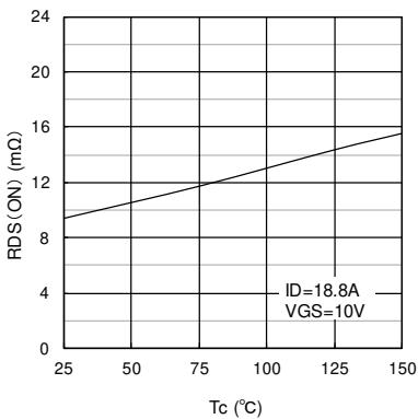
RDS(ON)-Tc characteristics (typical) ID=18.8A, VGS=10V
