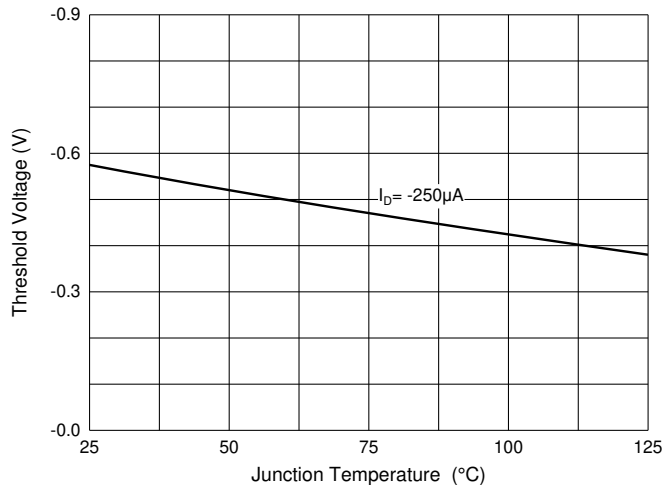
Fig. 6 - Threshold Voltage
