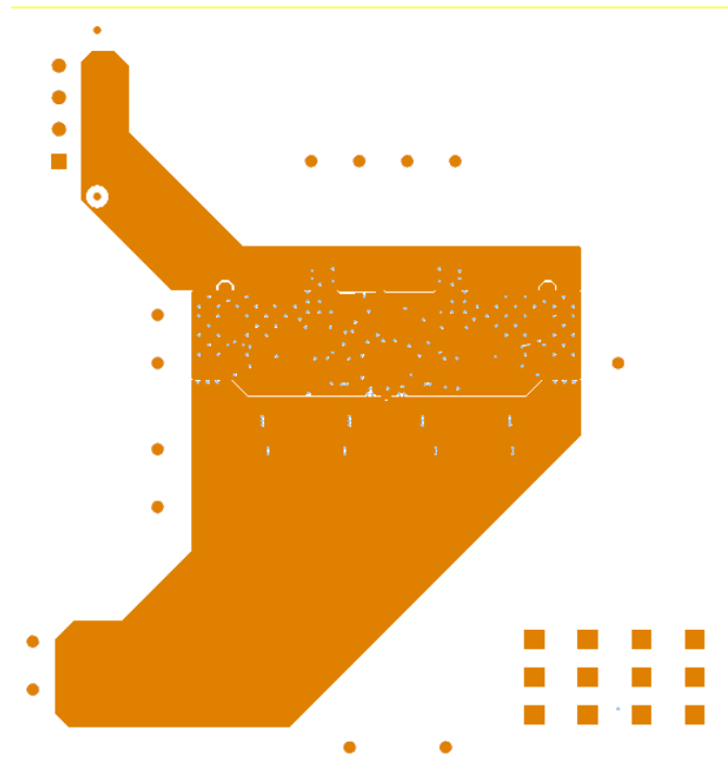
Fig. 7: Board layout, mid layer 3.
