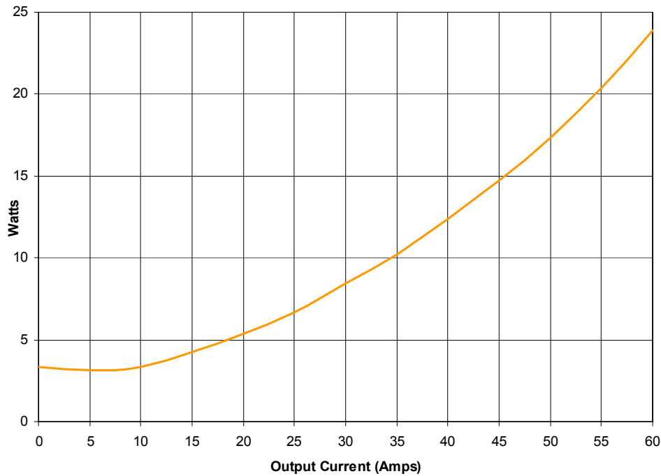
Fig. 34: Power loss versus load current at 45^\circ\text{C} with heat sink and 200LFM air flow
