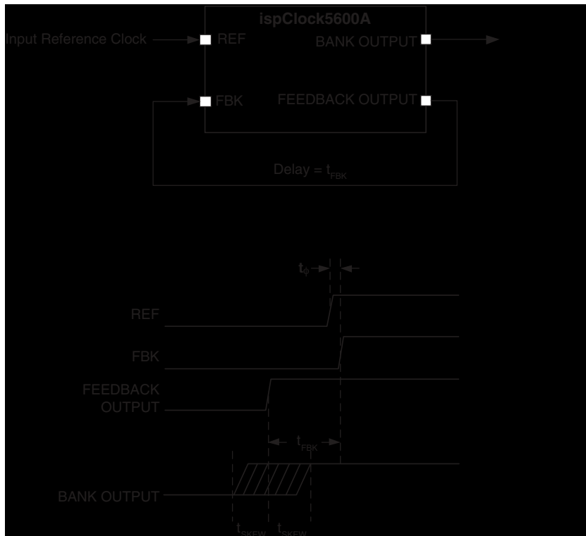
Figure 1-27. External Feedback Mode and Timing Relationships (Input, Output and Feedback Use the Same Logic Standard)
