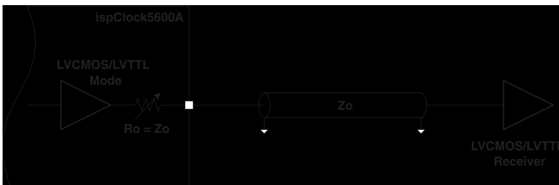
Figure 1-21. Configuration for LVTTTL/LVCMOS Output Modes
