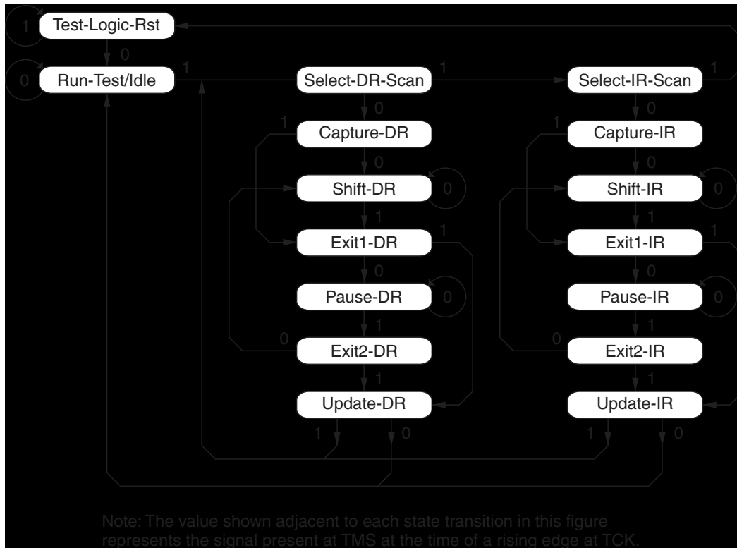
Figure 1-32. TAP States
