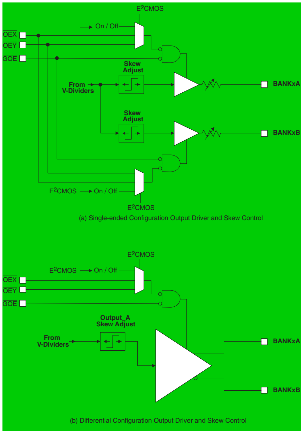
Figure 1-20. ispClock5600A Output Driver and Skew Control
