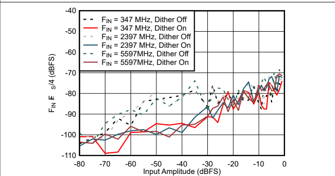
Figure 7-66. DES Mode: F_{\text{IN}} \pm F_S/4 vs Input Amplitude and Dither
