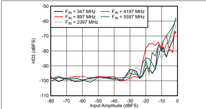
Figure 7-61. DES Mode: HD3 vs Input Amplitude and Frequency
