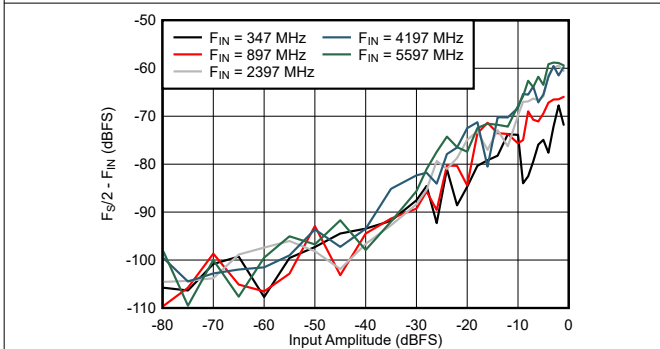
Figure 7-63. DES Mode: F_S/2 - F_{\text{IN}} vs Input Amplitude and Frequency
