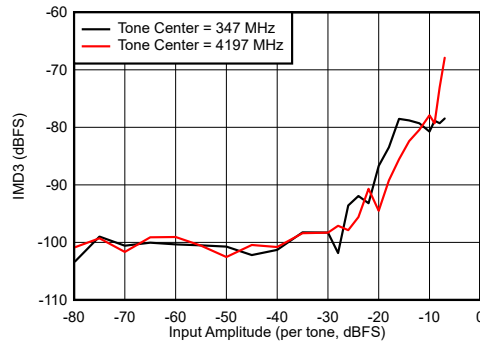
Figure 7-106. DES Mode: IMD3 vs Input Amplitude
