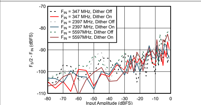
Figure 7-76. Dual Channel Mode: F_S/2 - F_{\text{IN}} vs Input Amplitude and Dither
