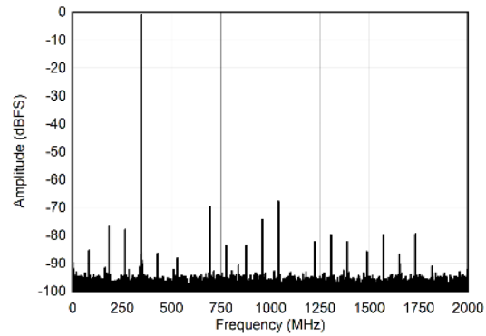
Figure 7-18. Dual Channel Mode: Single Tone FFT at 347 MHz
