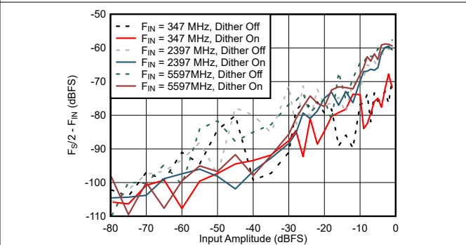
Figure 7-64. DES Mode: F_S/2 - F_{\text{IN}} vs Input Amplitude and Dither
