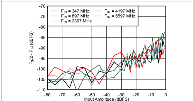
Figure 7-75. Dual Channel Mode: F_S/2 - F_{\text{IN}} vs Input Amplitude and Frequency
