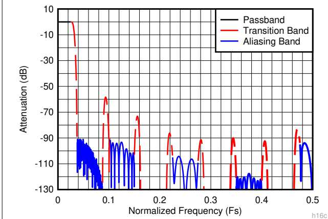
Figure 8-15. Decimate-by-16 Composite Response
