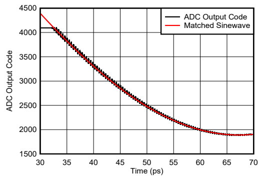
Figure 7-144. Sinewave Overdrive Recovery
