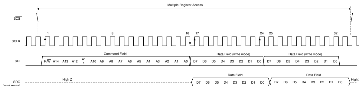
Figure 8-28. Serial Interface Protocol: Streaming Read/Write
