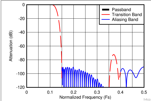
Figure 8-11. Decimate-by-4 Composite Response
