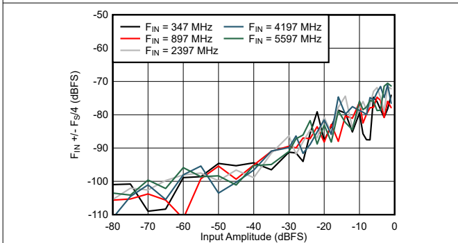
Figure 7-65. DES Mode: F_{\text{IN}} \pm F_S/4 vs Input Amplitude and Frequency
