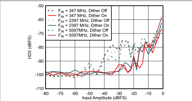
Figure 7-62. DES Mode: HD3 vs Input Amplitude and Dither
