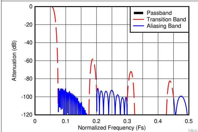
Figure 8-13. Decimate-by-8 Composite Response
