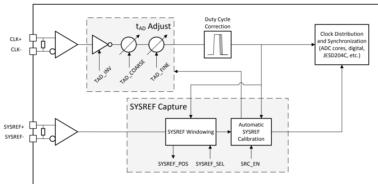
Figure 8-2. Clocking Subsystem
