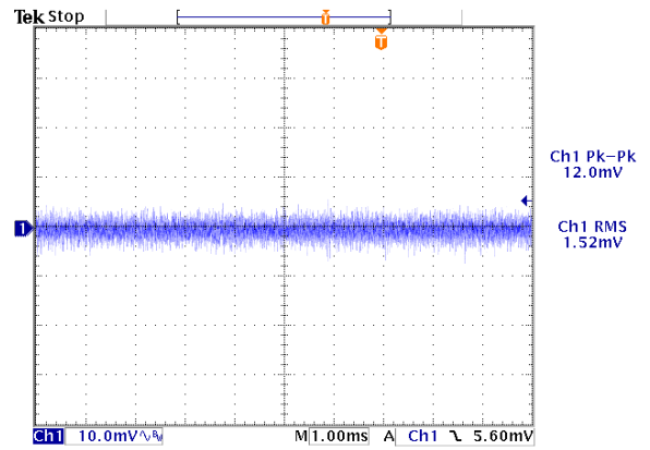
Figure 8: Output ripple & noise at 12Vin, 1.5V/80A out (10mv/div, 1mS/div)
