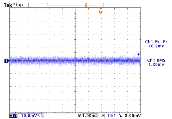
Figure 10: Output ripple & noise at 12Vin, 2.5V/80A out (10mv/div, 1mS/div)
