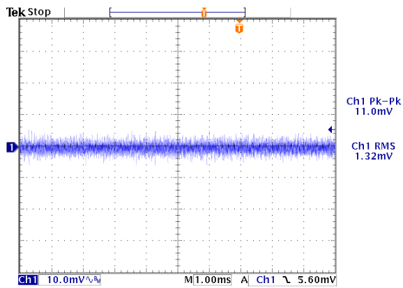
Figure 9: Output ripple & noise at 12Vin, 1.8V/80A out (10mv/div, 1mS/div)
