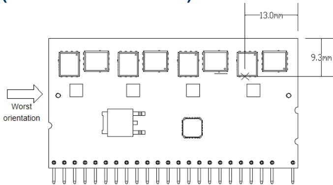
Figure 28: Hot spot temperature measured point
