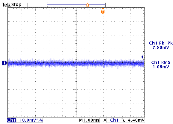
Figure 7: Output ripple & noise at 12Vin, 1.2V/80A out (10mv/div, 1mS/div)
