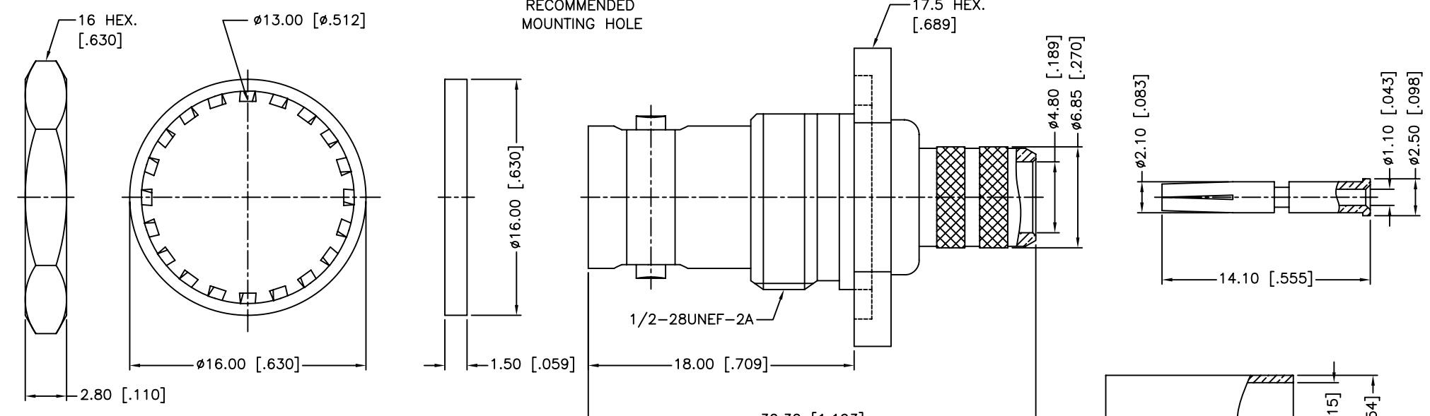
RECOMMENDED CABLE STRIPPING DIM'S
