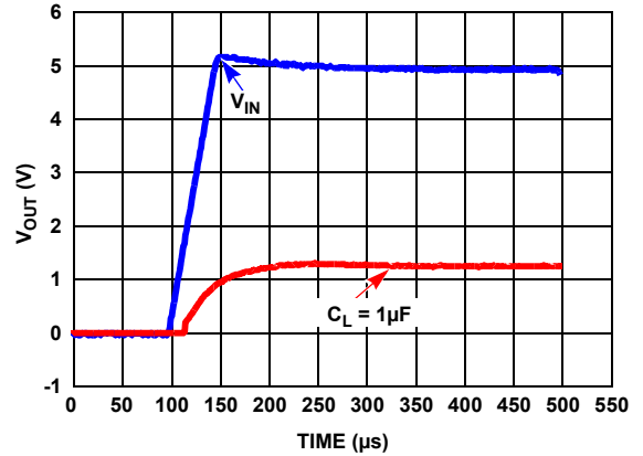
FIGURE 12. TURN ON TIME WITH 1 \mu\text{F}
