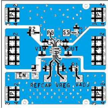
Figure 45. Typical Board Layout, Top Side
