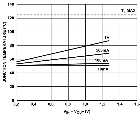
Figure 43. 1000 mm 2 of PCB Copper, T_B = 50^\circ\text{C}
