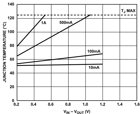
Figure 39. 25 mm 2 of PCB Copper, T A = 50°C
