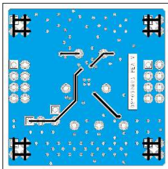
Figure 46. Typical Board Layout, Bottom Side
