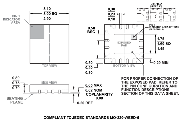
COMPLIANT TO JEDEC STANDARDS MO-220-WEED-6 Figure 47. 16-Lead Lead Frame Chip Scale Package [LFCSP] 3 mm x 3 mm Body and 0.75 mm Package Height (CP-16-22) Dimensions shown in millimeters
