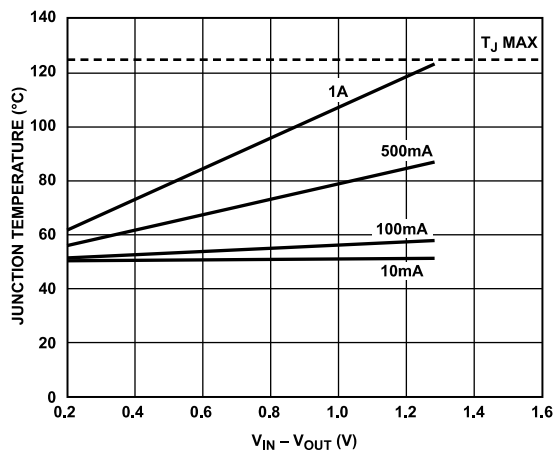
Figure 37. 6400 mm 2 of PCB Copper, T A = 50°C
