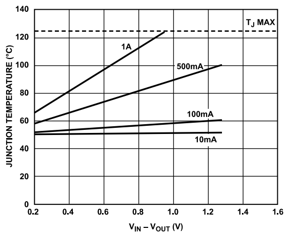
Figure 38. 500 mm 2 of PCB Copper, T A = 50°C
