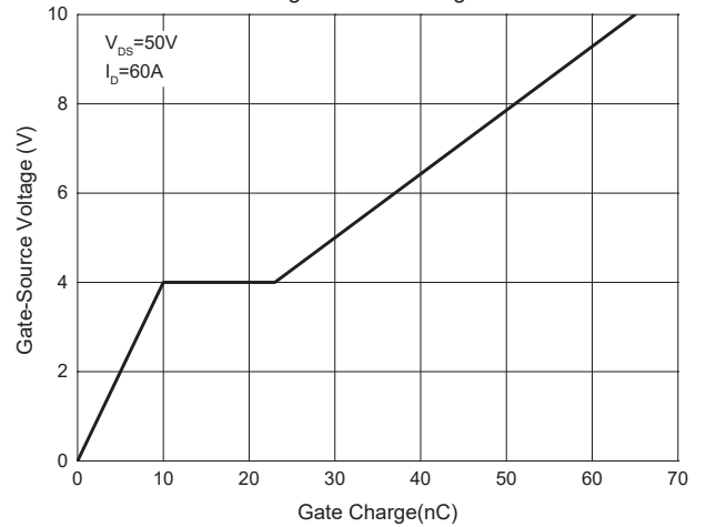
Fig. 4 - Gate Charge
