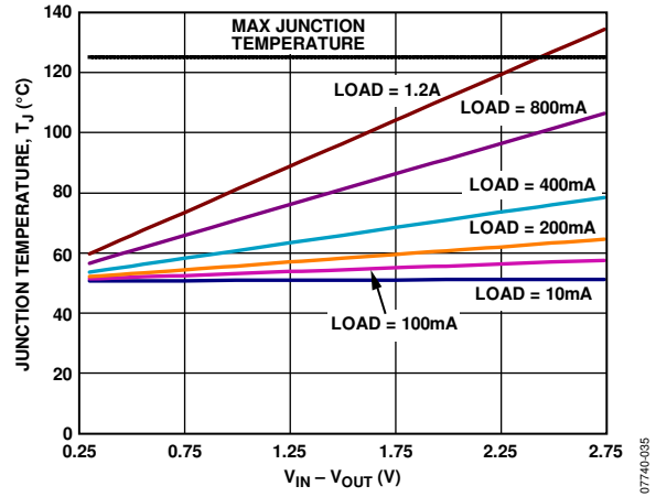
Figure 20. 1000 mm 2 of PCB Copper, T B = 50°C, LFCSP
