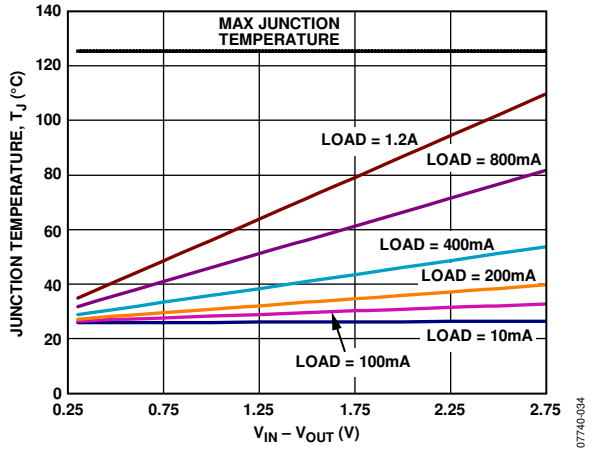
Figure 19. 1000 mm 2 of PCB Copper, T B = 25°C, LFCSP
