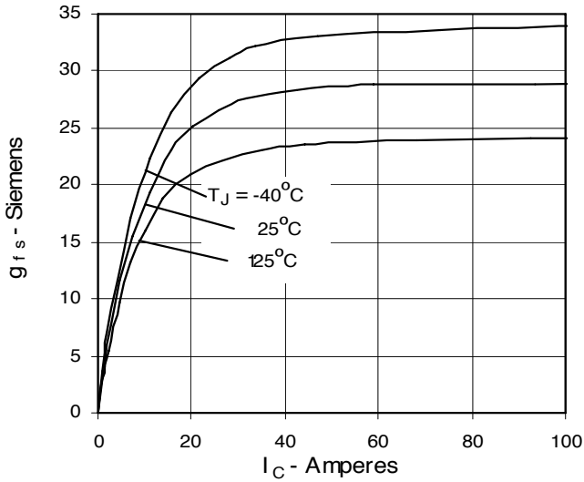
Fig. 7. Transconductance
