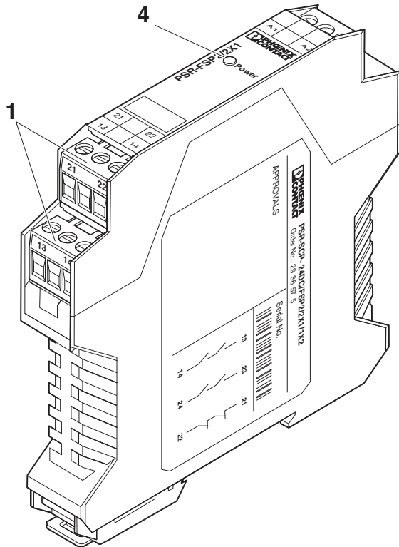
Figure 5 PSR-SCP- 24DC/FSP2/2X1/1X2
