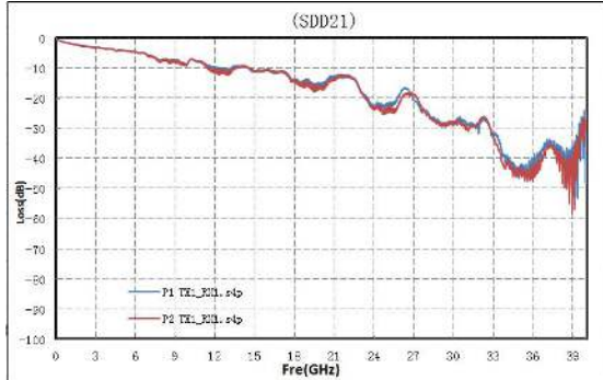
SFP28 30AWG 1M
