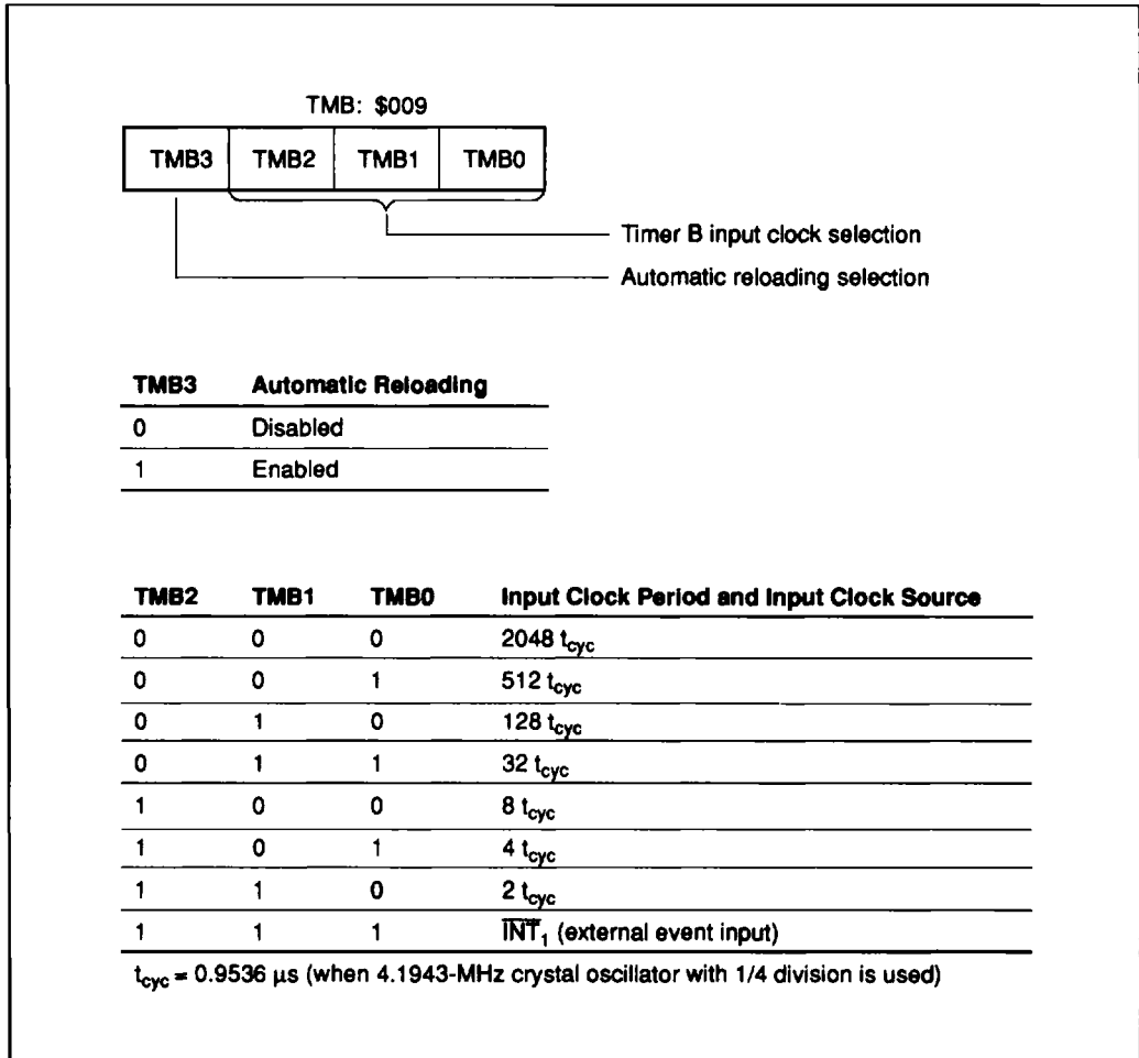
Figure 30 Timer Mode Register B
