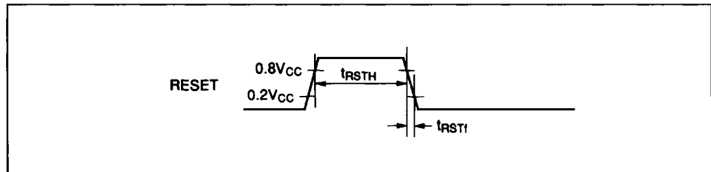
Figure 60 Reset Timing
