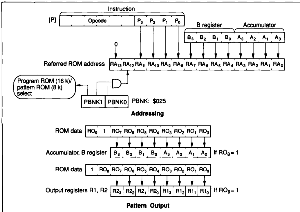
Figure 54-2 P Instruction (HD404720, HD4074720)
