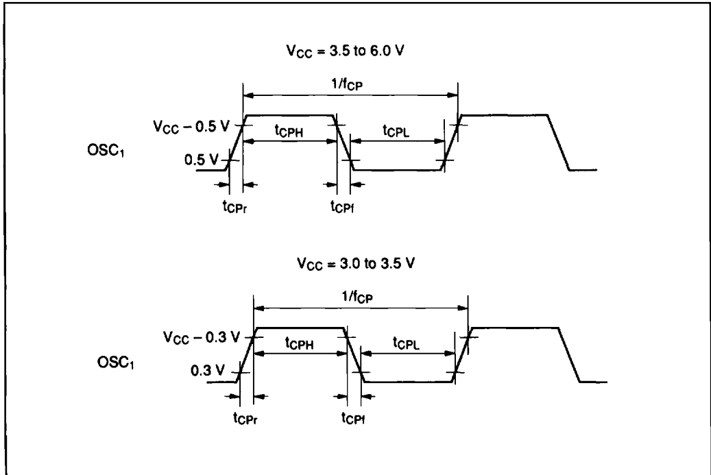
Figure 58 Oscillator Timing
