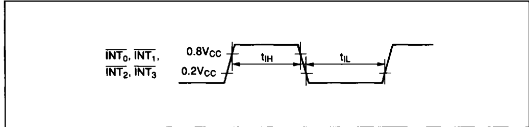
Figure 59 Interrupt Timing
