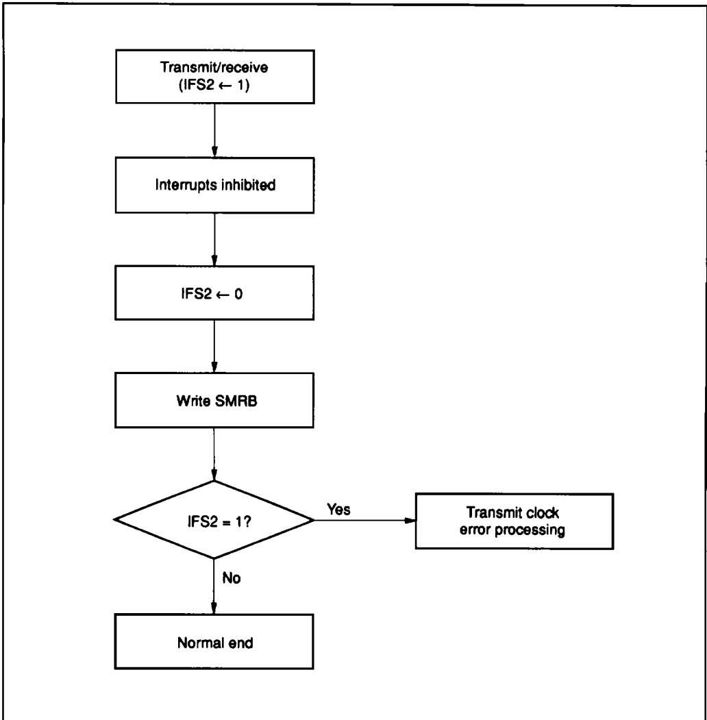
Figure 41 Transmit Clock Error Detection
