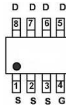
pin assignment
