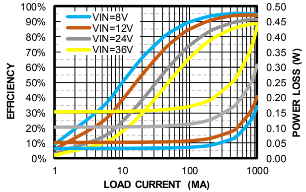
Efficiency vs. Load Current vs. Power Loss V OUT = 3.3V, FCCM
