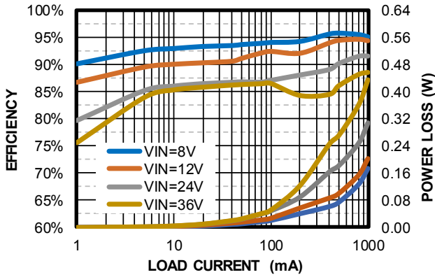
Efficiency vs. Load Current vs. Power Loss V OUT = 3.3V, AAM mode
