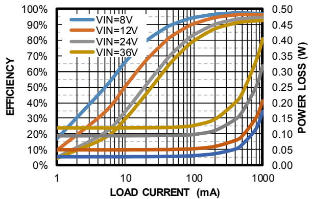
Efficiency vs. Load Current V OUT = 5V, FCCM
