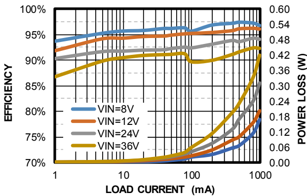
Efficiency vs. Load Current vs. Power Loss V OUT = 5V, AAM mode
