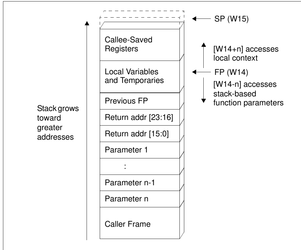
FIGURE 4-4: PUSH CALLEE-SAVED REGISTERS
