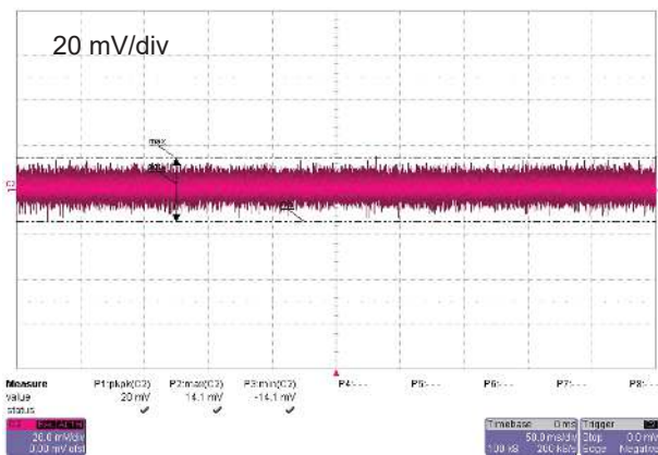
Figure 15: Output noise
