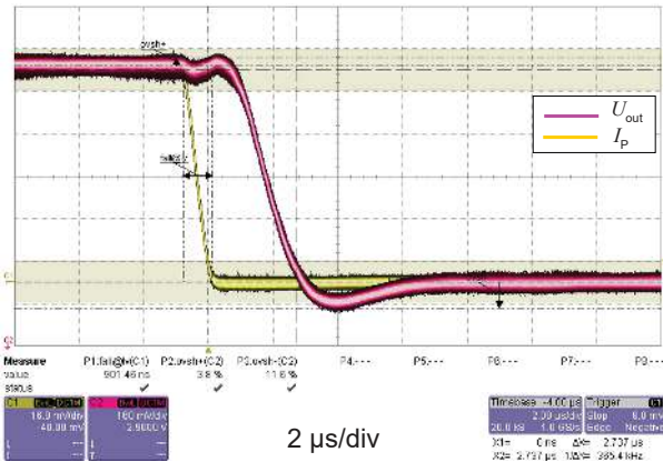
Figure 3: Step response
