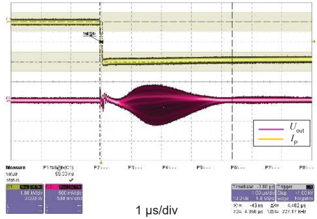
Figure 9: dv/dt
