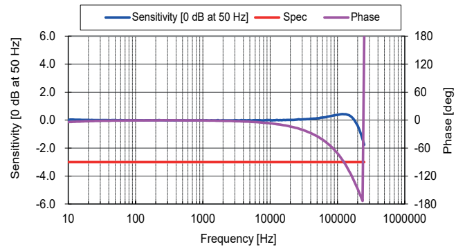
Figure 7: Frequency response
