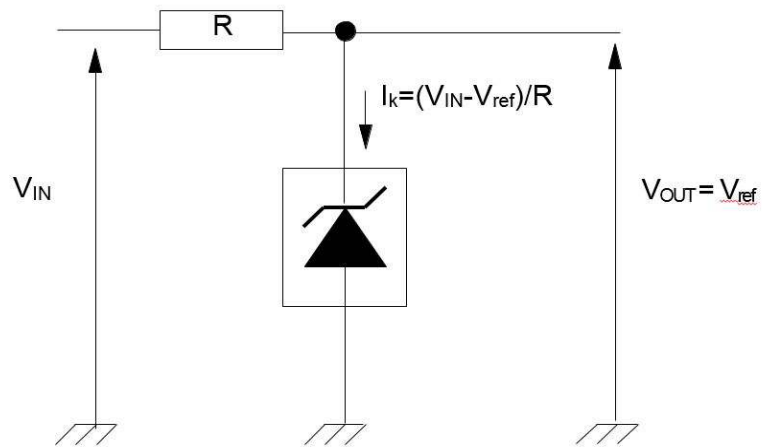
Figure 2. Application circuit
