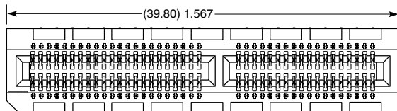
40 POSITIONS
