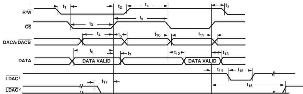
Figure 2. Timing Diagram
