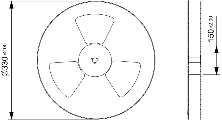
PLASTIC REEL (BLACK): 477995358 (WITH EMPTY CARRIER IN)
