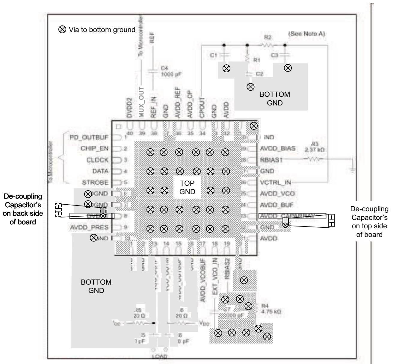
Figure 89. TRF3761 Layout
