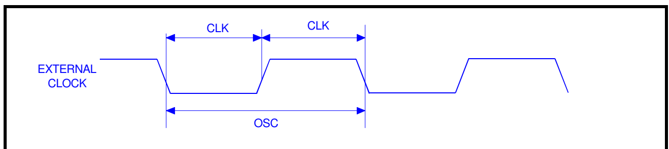
FIGURE 16. CLOCK TIMING
