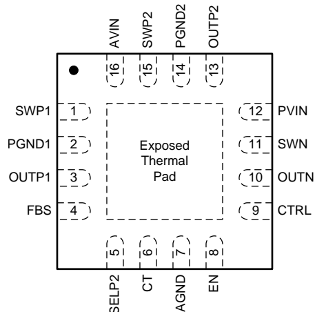
Pin Functions
