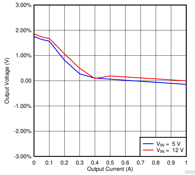
Figure 4-3. Load Regulation
