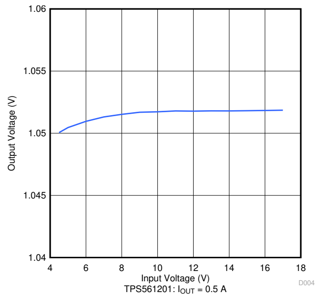
Figure 4-4. Line Regulation
