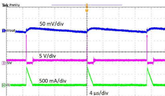
Figure 4-8. Output Voltage Ripple, I_{OUT} = 10\text{ mA}
