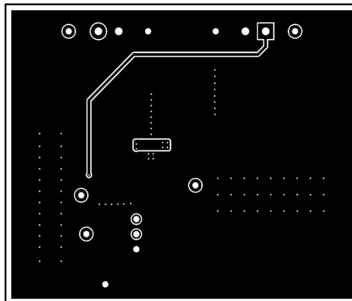
Figure 5-3. Bottom Layer
