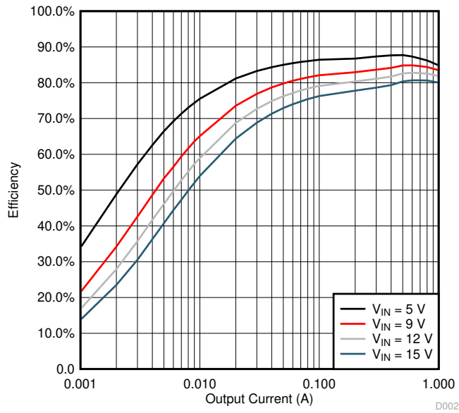
Figure 4-2. Light-Load Efficiency
