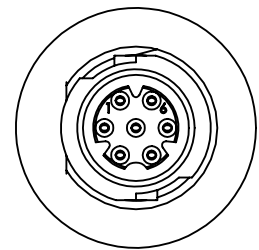
FACE VIEW W17984-7SG-P-300 7 POSITION A-KEY
