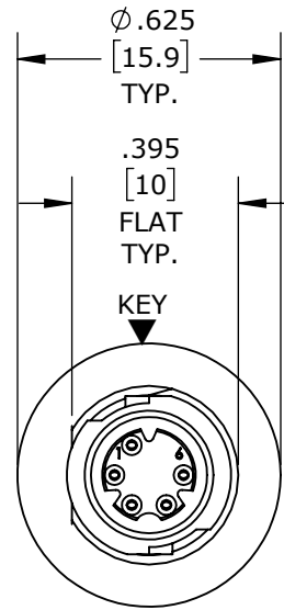
FACE VIEW W17984-5SG-P-300 5 POSITION A-KEY
