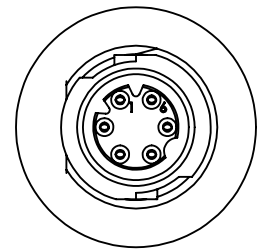
FACE VIEW W17984-6SG-P-300 6 POSITION B-KEY
