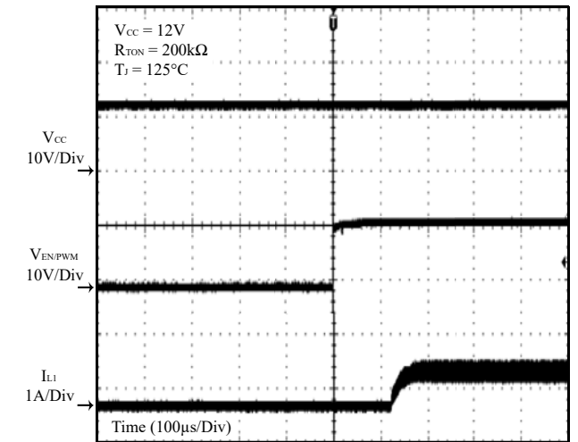
Figure 20 EN/PWM Enable Time
