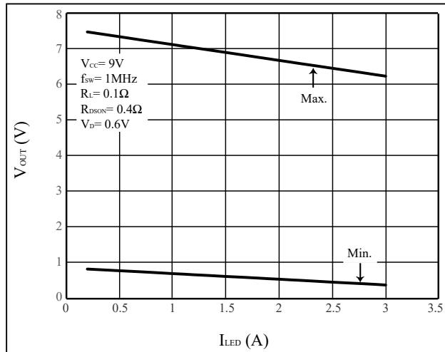
Figure 33 Minimum and Maximum Output Voltage versus LED Current (minimum t_{ON} and t_{OFF} = 150\text{ns} )
