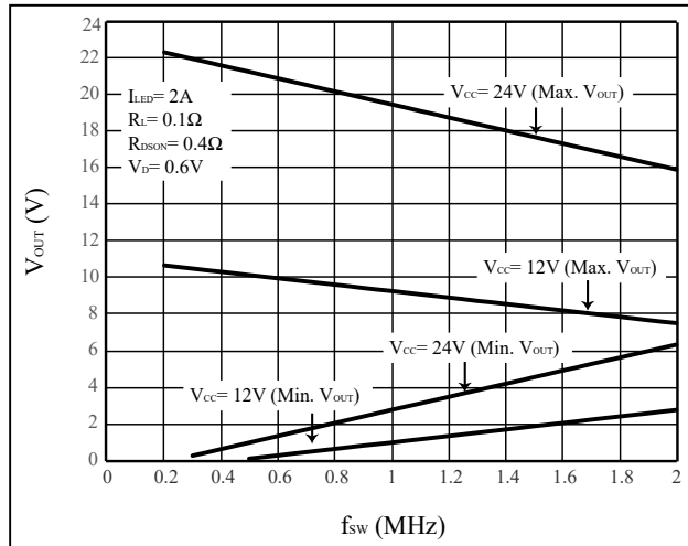
Figure 32 Minimum and Maximum Output Voltage versus Operating Frequency (minimum t_{ON} and t_{OFF} = 150\text{ns} )
