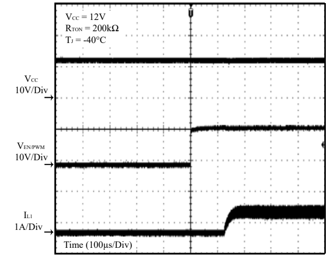
Figure 18 EN/PWM Enable Time
