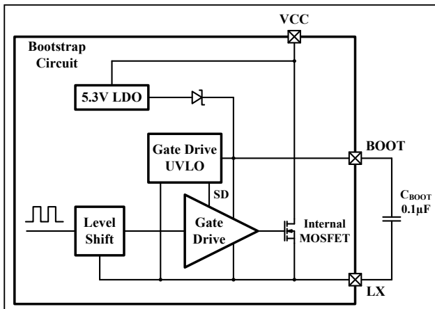
Figure 27 Bootstrap Circuit
