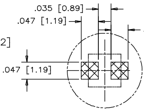
DETAIL 'A' (ENLARGED) SMT LED SOLDER PAD (SMT LED TO BE PROVIDED BY THE CUSTOMER)
