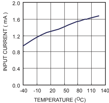
Input Supply Current vs. Temp
