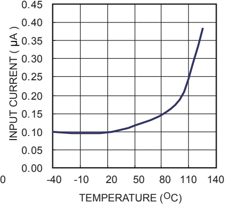
Shut Down Input Current vs. Temp
