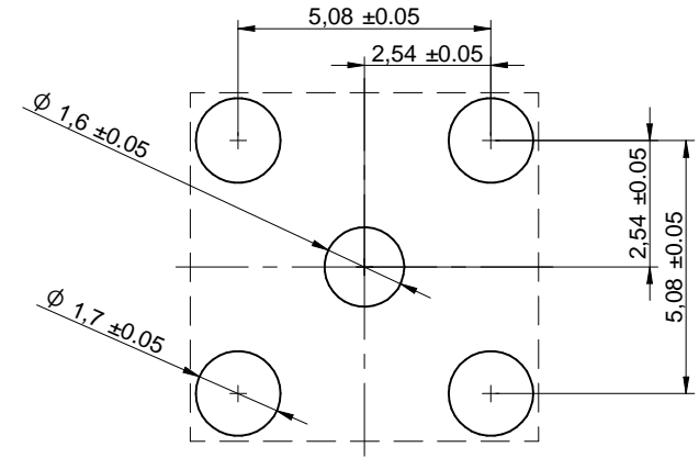
Scale 6:1
