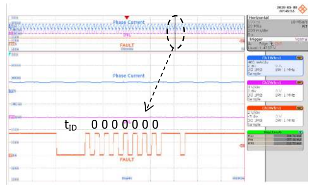
Figure 39 – External Temperature Fault Cleared. Status Update: 000 00 0 0 (Fault Clear). Upper: I_{MOTOR} , 400 mA / div. Middle: V_{INL\_U} , 4 V / div. Lower: V_{FAULT} , 2 V / div., 200 ms / div. Zoom: 50 \mu s / div
