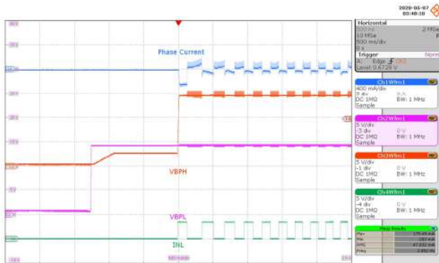
Figure 5 – BPL and BPH-pin Voltages at Start-Up First: I_{MOTOR} , 400 mA / div. Second: V_{BPH} , 5 V / div. Third: V_{BPL} , 5 V / div. Fourth: V_{INL} , 5 V / div. Time Scale: 500 ms / div.
