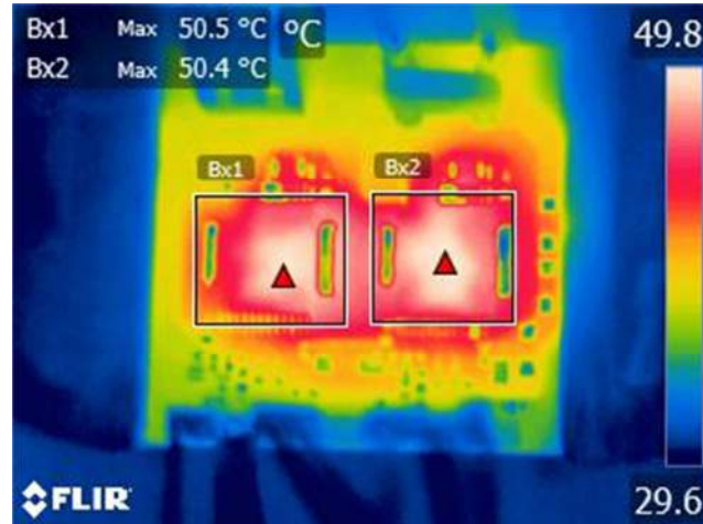
Figure 19 – Thermal Scan at 15 W Inverter Output in Self-Supply Operation.
