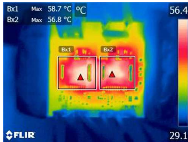
Figure 20 – Thermal Scan at 30 W Inverter Output in Self-Supply Operation.
