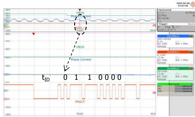
Figure 33 – Bus Sensing - Brown-out. Bus Voltage Drop 240 to 200 VDC. Status Update: 011 00 0 0 (UV85). Upper: V_{BUS} , 50 V / div. Middle: I_{MOTOR} , 400 mA / div. Lower: V_{FAULT} , 2 V / div., 50 ms / div. Zoom: 50 \mu s / div.
