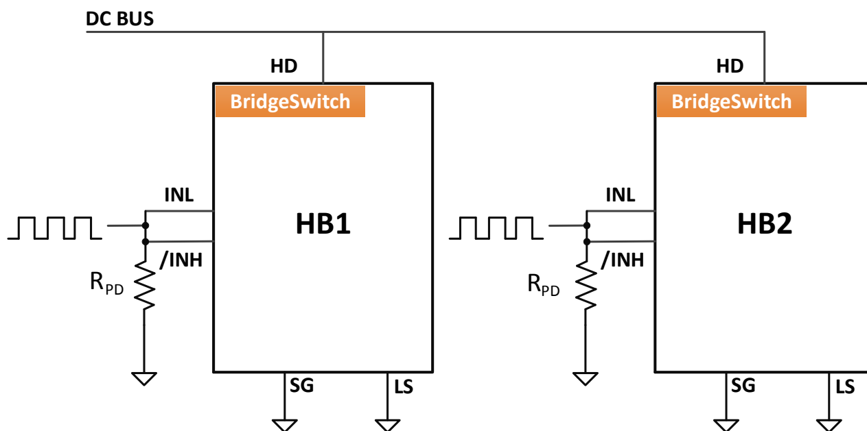
Figure 58 – Complementary PWM Signal Implementation with BridgeSwitch Inverter.
