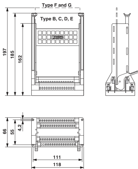
Dimensioned drawing
