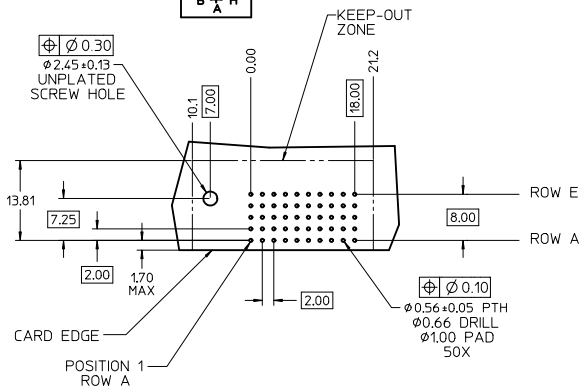
DAUGHTERCARD HOLE PATTERN (CONNECTOR SIDE)
