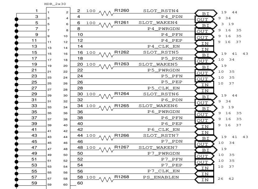
PORTS 4, 5, 6, 7
