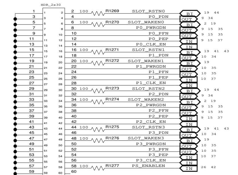
PORTS 0, 1, 2, 3
