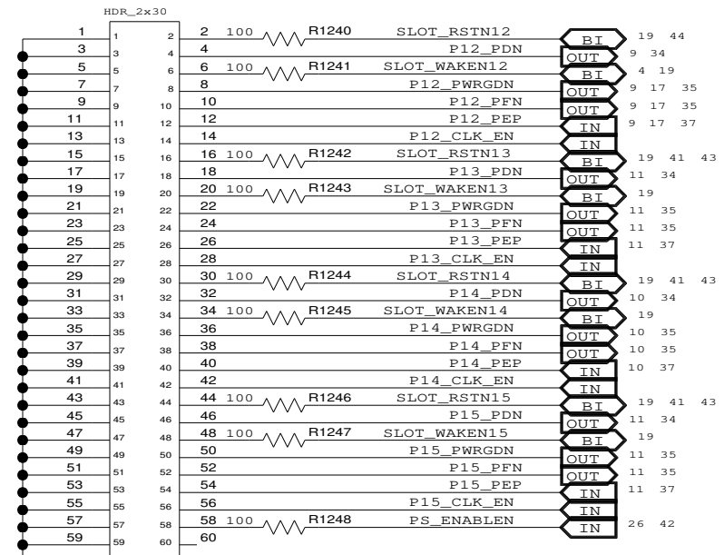
PORTS 12, 13, 14, 15
