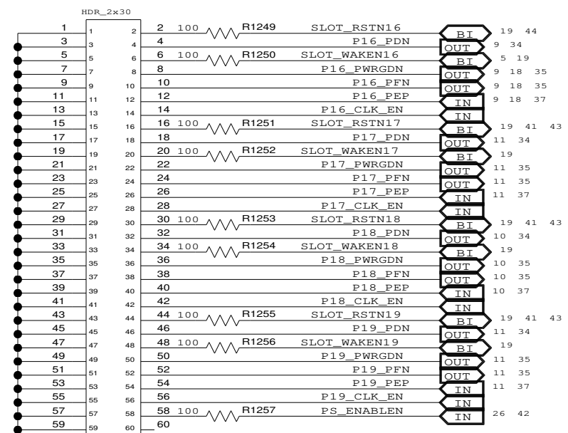
PORTS 16, 17, 18, 19
