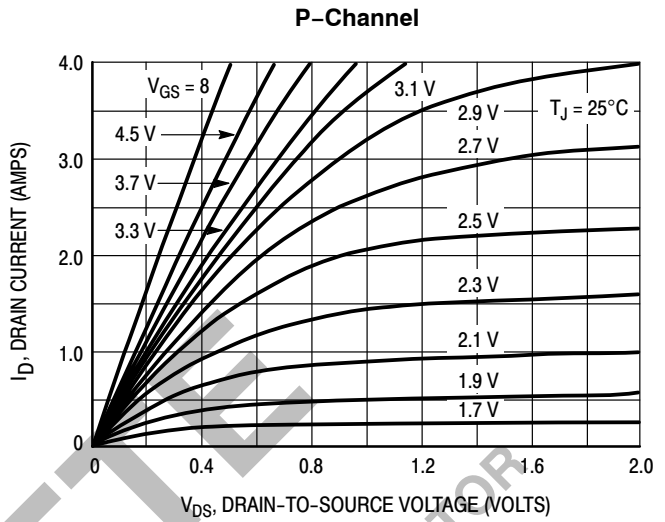
Figure 1. On-Region Characteristics
