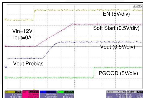
Figure 17. FAN23SV06 Startup Waveforms with Pre-Bias Voltage on Output
