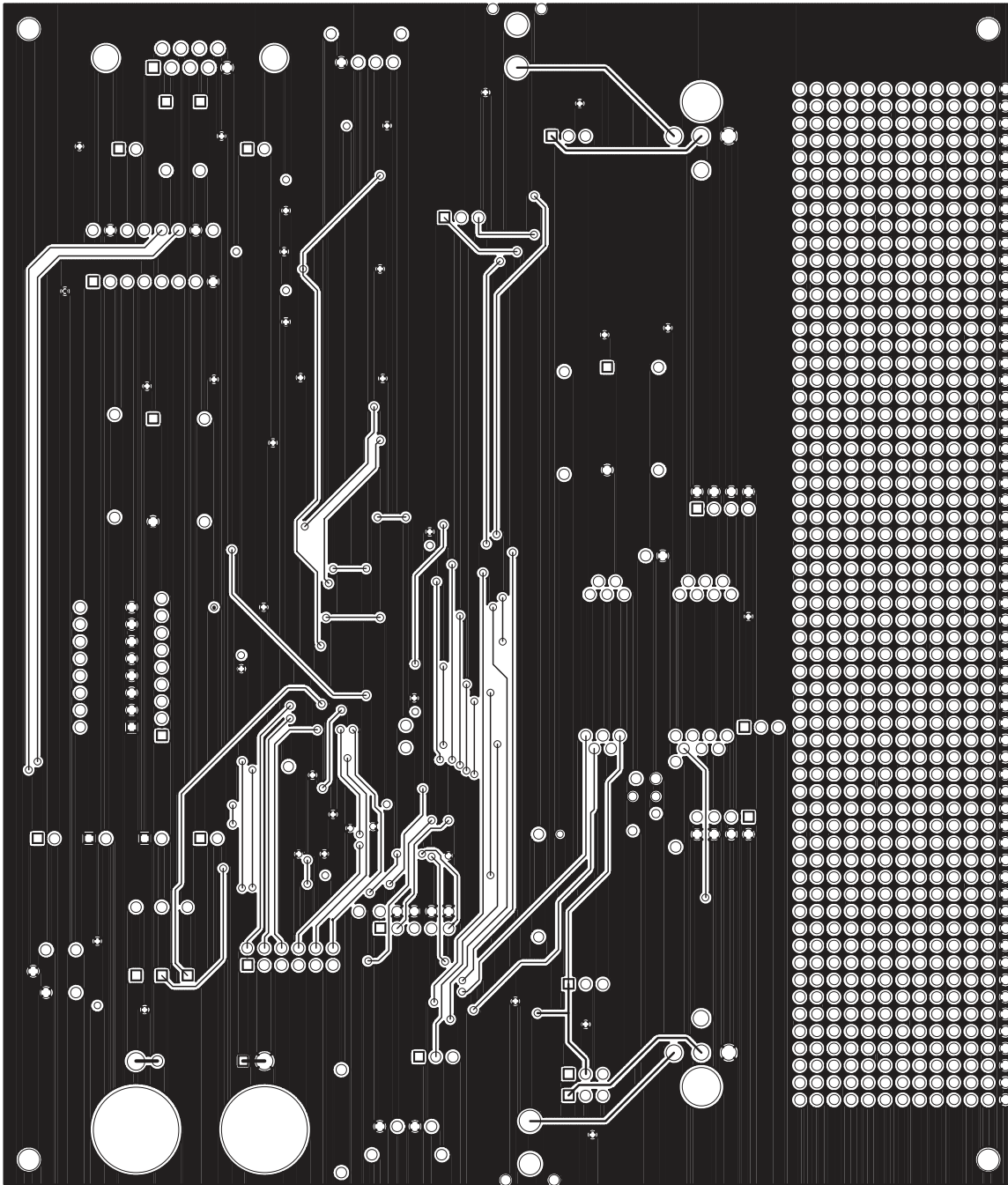
Figure 8. Bottom PCB
